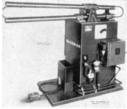
Left: The Eisler automatic motor-driven spot welder. (Patent No. 2,006,544.) Right: The Eisler long-horn air-operated spot welder, adjustable for various sizes of spot welding with the 12" to 48" throat depth and long arms (15 to 75 K.V.A.). (Patent No. 2,231,617.)
